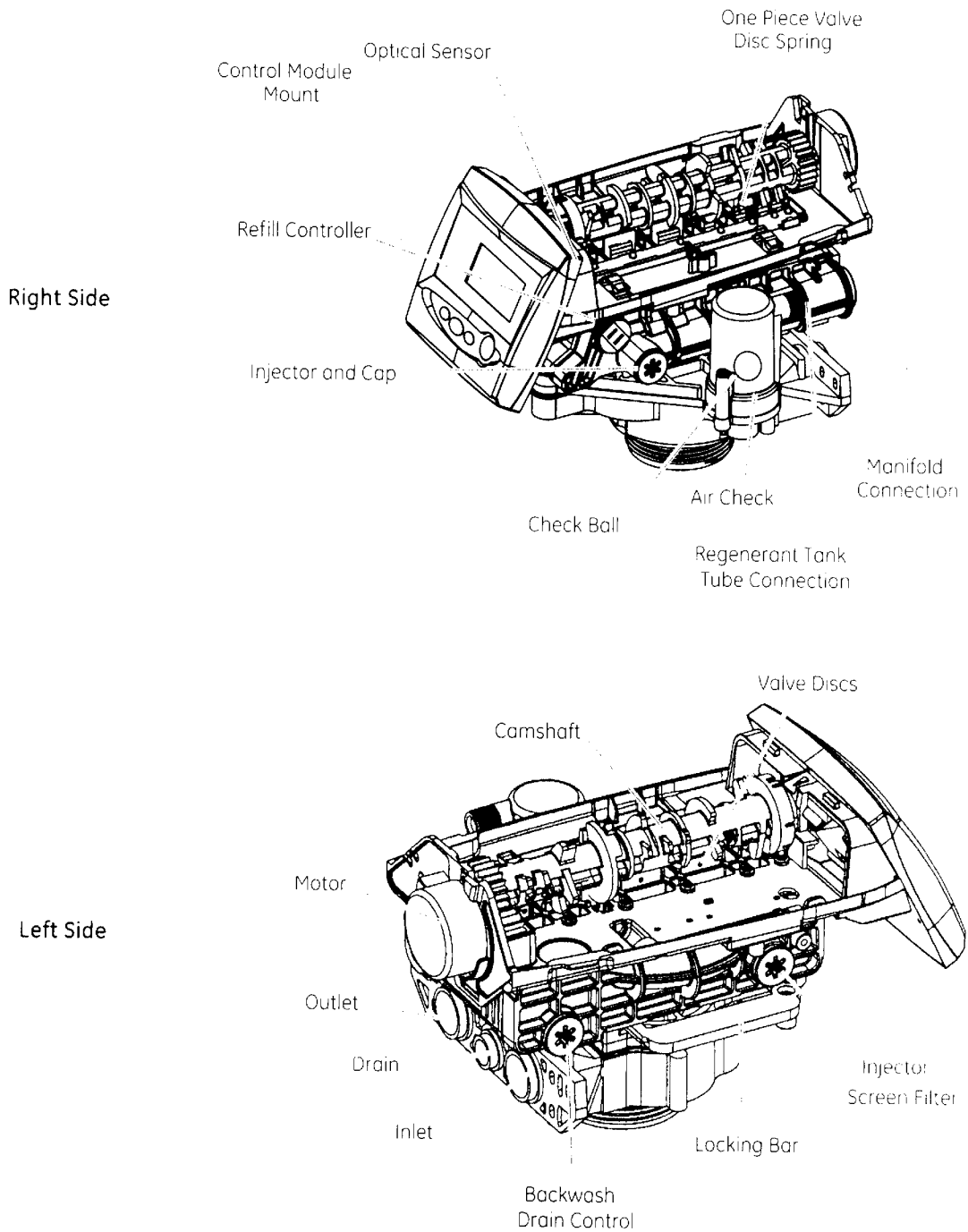
Figure 2 255 Valve Identification
